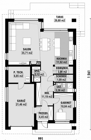
E-255a PARTER
