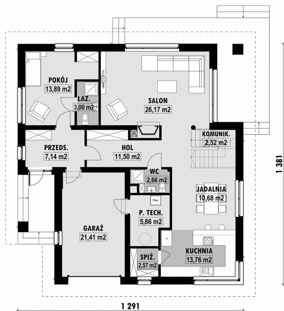
E-228 PARTER
