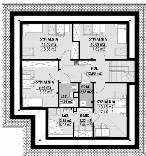
E-228 PODDASZE
