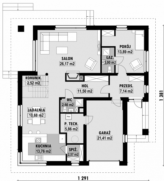
E-228-L PARTER
