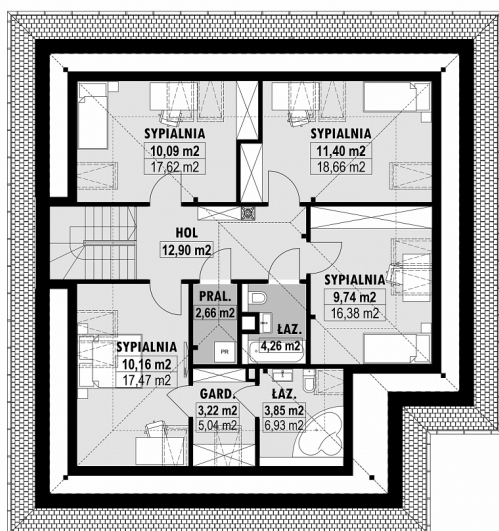
E-228-L PODDASZE
