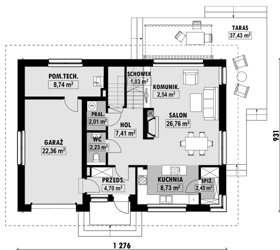
E-290a PARTER
