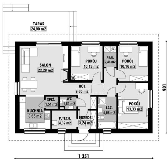
E-281-L PARTER
