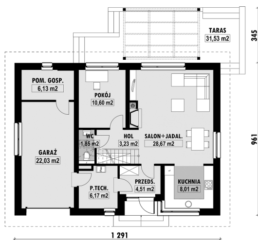
E-279 PARTER
