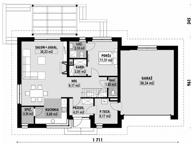
E-277-L PARTER
