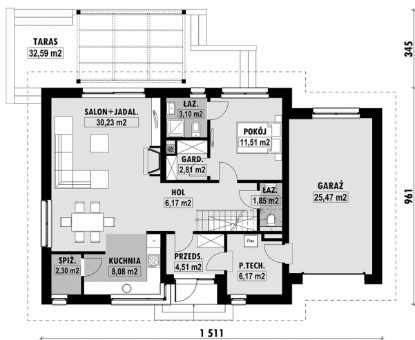
E-276-L PARTER
