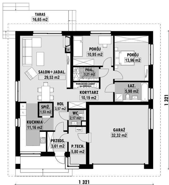
E-268a-L PARTER
