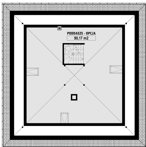
E-268a-L PODDASZE
