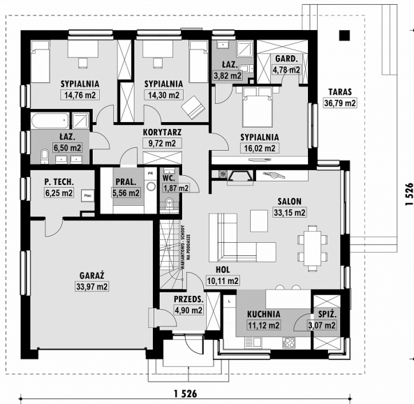
E-264a-L PARTER
