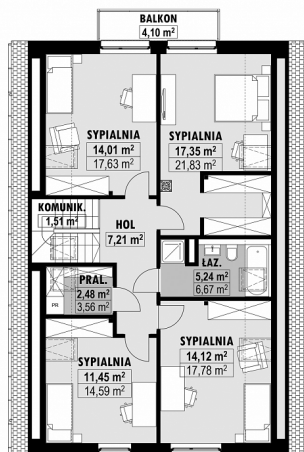
E-258-L PODDASZE
