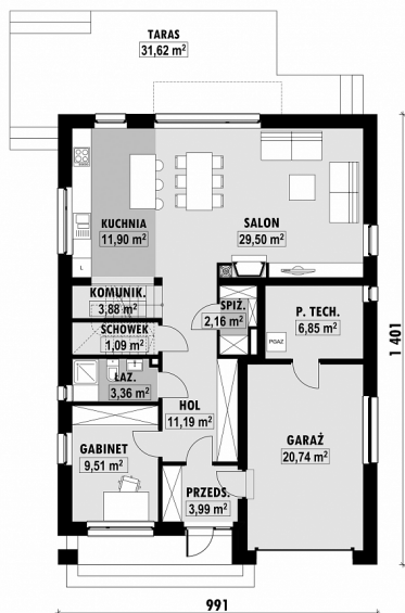
E-258-L PARTER
