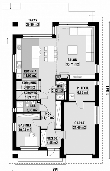
E-255a-L PARTER
