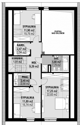
E-255a-L PODDASZE
