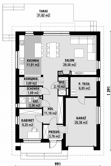
E-254-L PARTER
