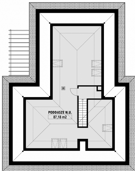
E-250-L PODDASZE
