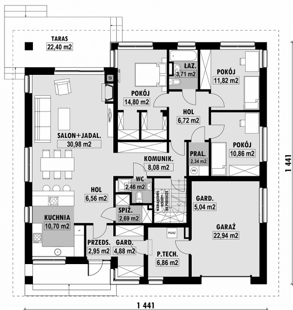
E-240-L PARTER
