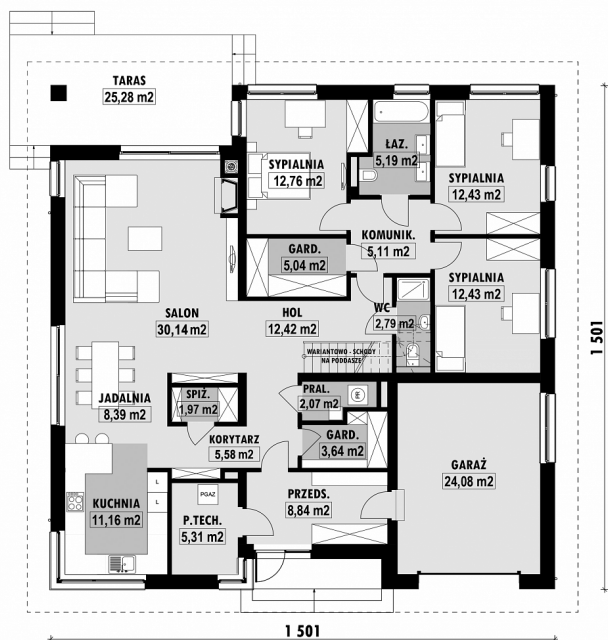
E-239-L PARTER
