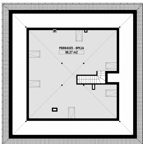
E-239-L PODDASZE
