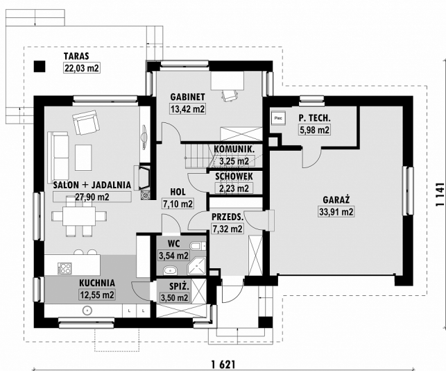
E-237-L PARTER
