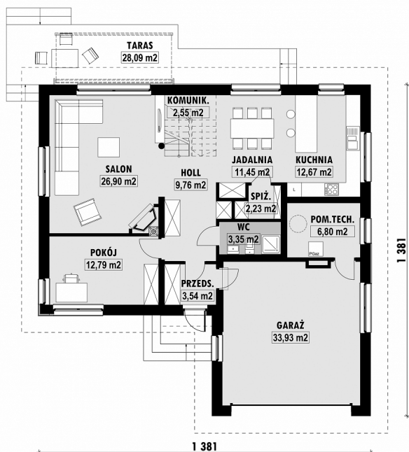
E-224-L PARTER
