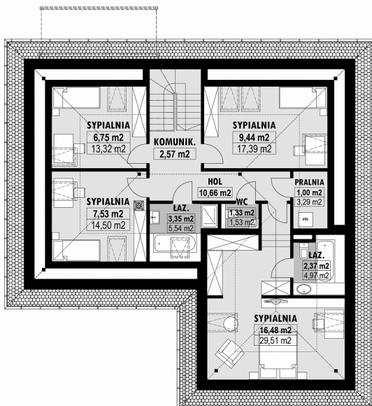
E-224-L PODDASZE
