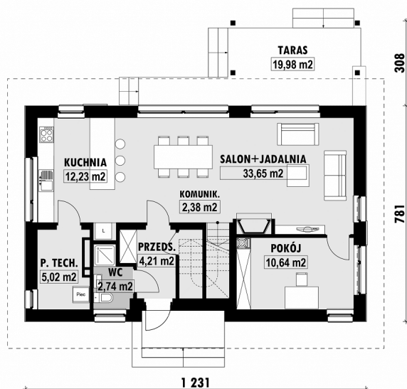
E-222 PARTER
