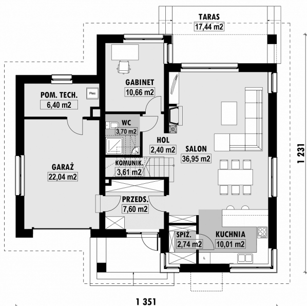
E-208 PARTER
