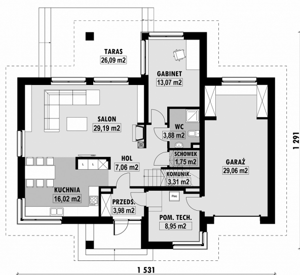
E-190-L PARTER
