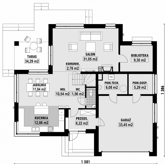
E-187-L PARTER
