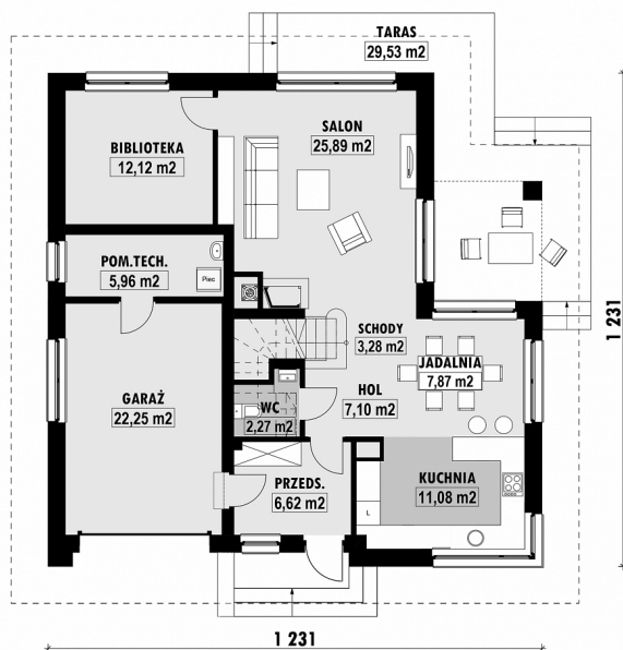
E-177 PARTER
