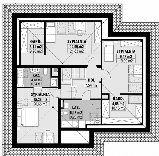
E-168 PODDASZE
