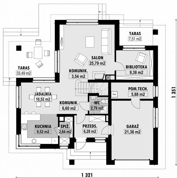
E-167-L PARTER
