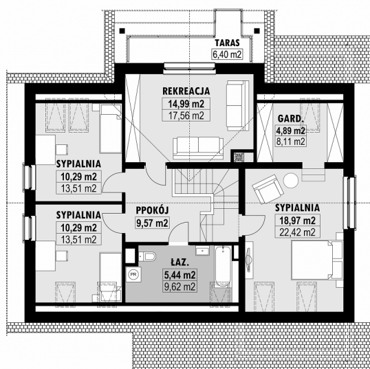
E-167-L PODDASZE
