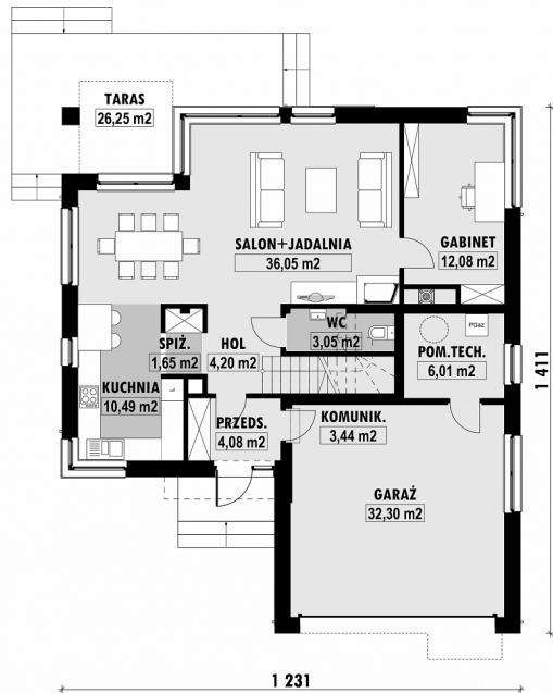
E-162-L PARTER
