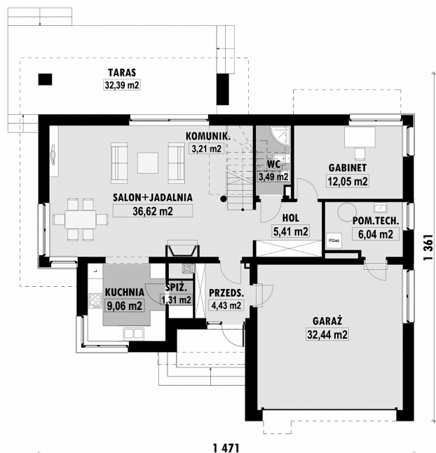
E-123-L PARTER
